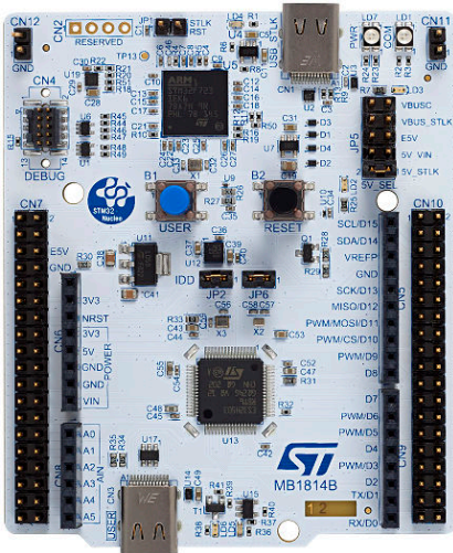
NUCLEO-H503RB example. Boards with different references show different layouts. Picture is not contractual.
