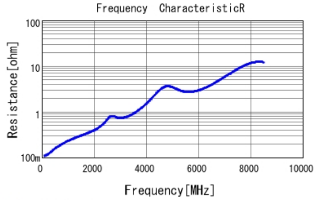
GCM1885C2A330JA16 R DCOV, 25degC
