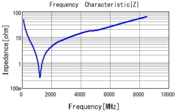
GCM1885C2A330JA16 |Z| DCOV, 25degC
