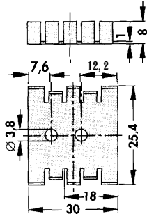
FK 21 O/SA-CB 18 K/W
