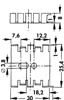
FK 212/CB ... 18 K/W
