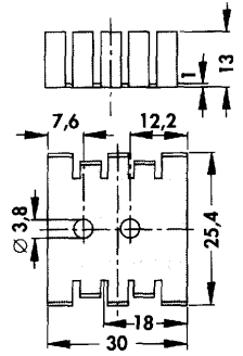
FK 214/SA-CB 15 K/W
