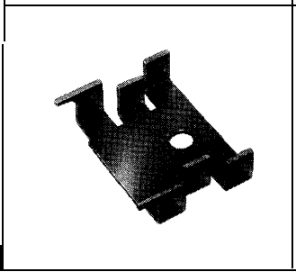
FK 21 1/32 ... 25 K/W
