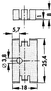
FK 209/SA-32 25 K/W
