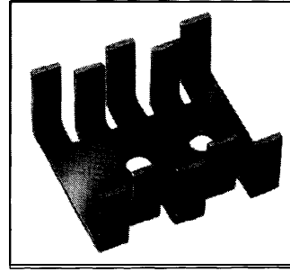
FK 214/SA-CB 15 K/W
