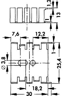
FK 214/CB ... 15 K/W
