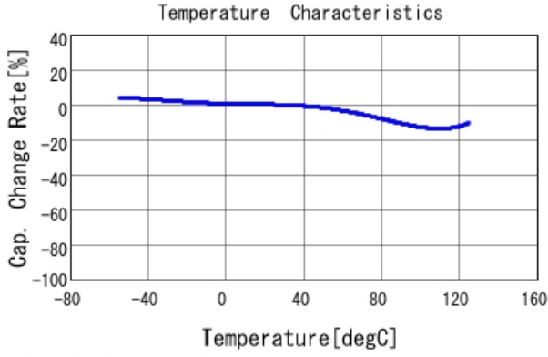
■ GRM55DR72E684KW01 C-Temp. capchange, DCOV, AC1Vrms
