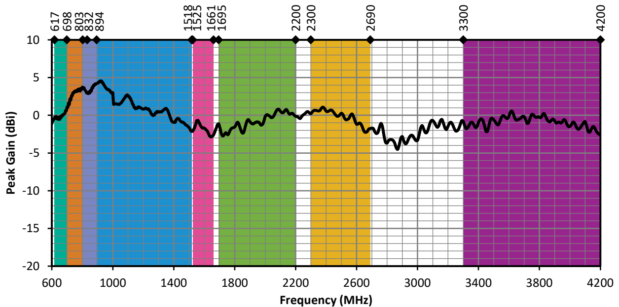
Figure 13. ANT-5GW-MMG1-SMA Peak Gain, Free Space
