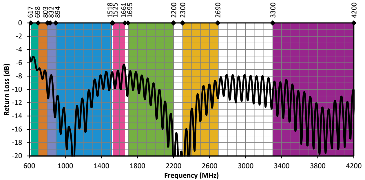
Figure 12. ANT-5GW-MMG1-SMA Return Loss, Free Space
