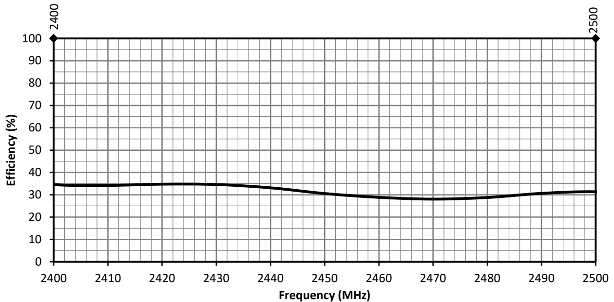
Figure 8. ANT-2.4-MMG1-SMA Antenna Radiation Efficiency on Ground Plane
