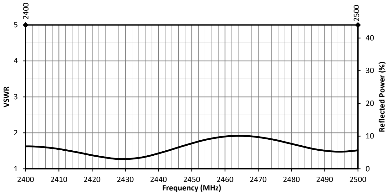
Figure 4. ANT-2.4-MMG1-SMA Antenna VSWR on Ground Plane
