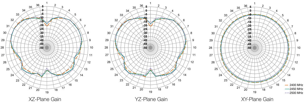
Figure 16. Radiation Patterns for ANT-2.4-MMG1-SMA Antenna, Free Space
