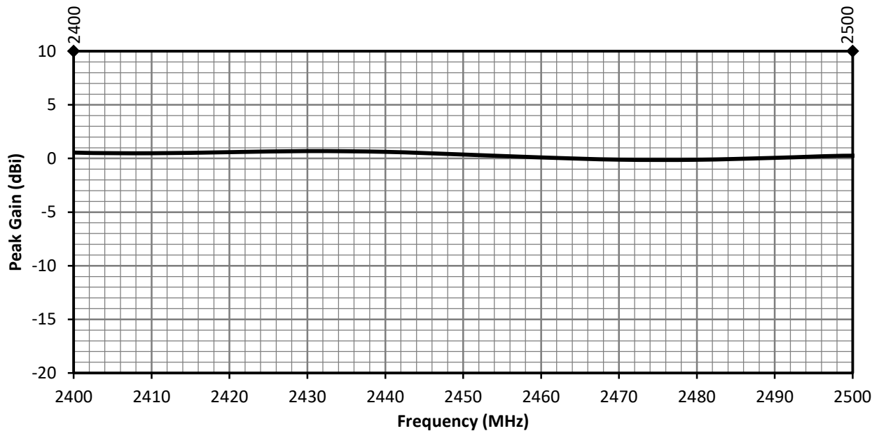
Figure 13. ANT-2.4-MMG1-SMA Antenna Peak Gain, Free Space
