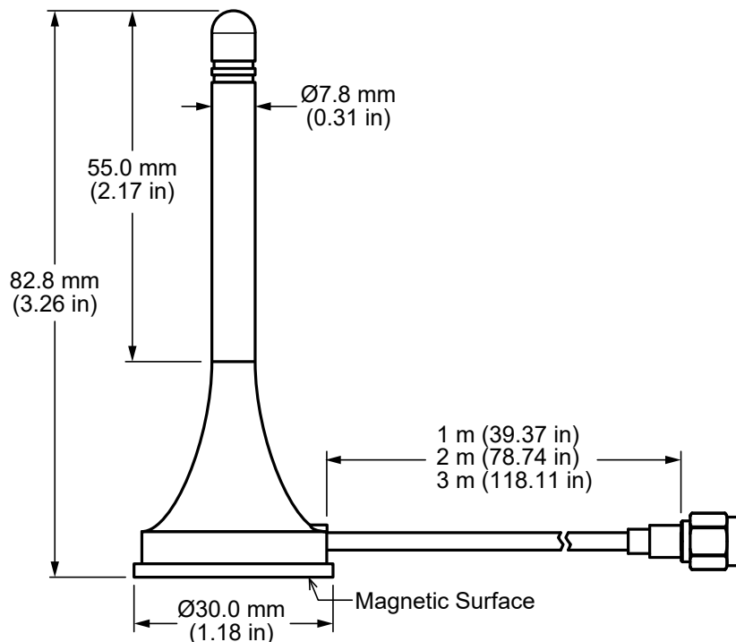
Figure 1. ANT-2.4-MMG1-SMA Series Antenna Dimensions
