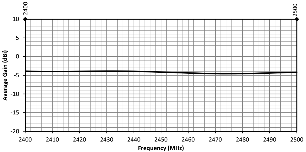
Figure 14. ANT-2.4-MMG1-SMA Antenna Average Gain, Free Space
