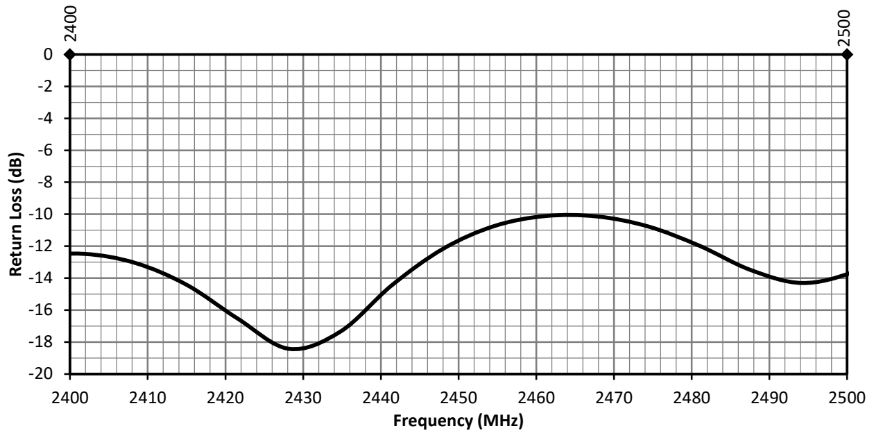
Figure 5. ANT-2.4-MMG1-SMA Antenna Return Loss on Ground Plane
