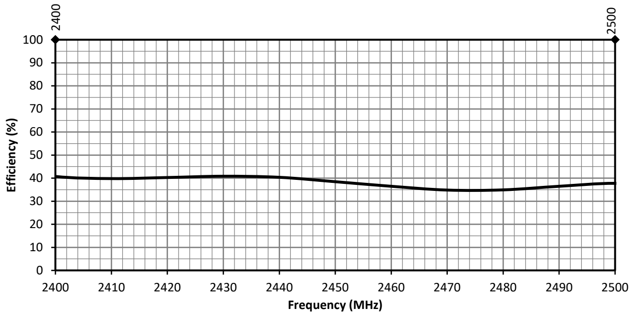
Figure 15. ANT-2.4-MMG1-SMA Antenna Radiation Efficiency, Free Space
