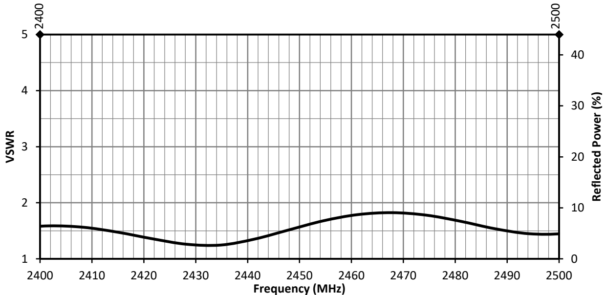
Figure 11. ANT-2.4-MMG1-SMA Antenna VSWR, Free Space
