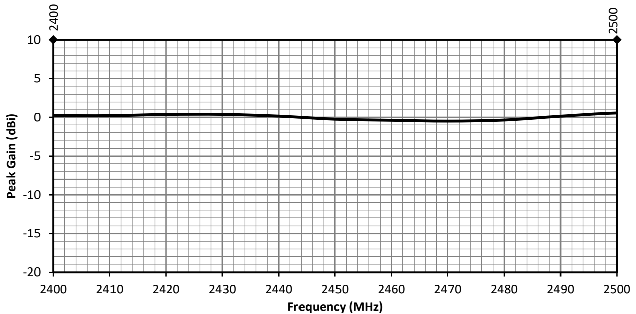
Figure 6. ANT-2.4-MMG1-SMA Antenna Peak Gain at Center of Ground Plane
