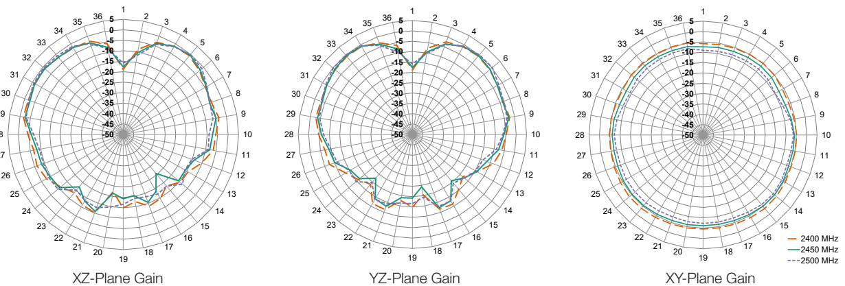
Figure 9. Radiation Patterns for ANT-2.4-MMG1-SMA Antenna on Ground Plane
