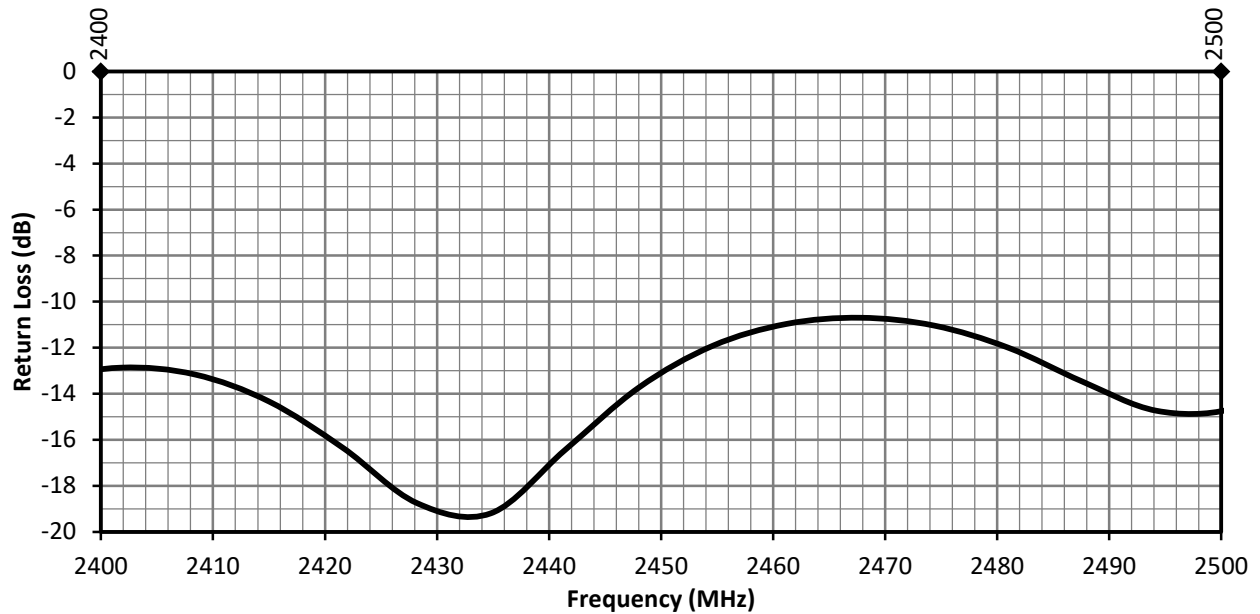
Figure 12. ANT-2.4-MMG1-SMA Antenna Return Loss, Free Space
