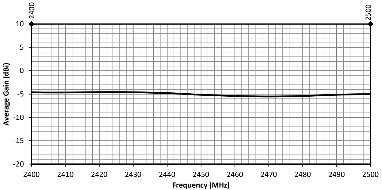
Figure 7. ANT-2.4-MMG1-SMA Antenna Average Gain on Ground Plane
