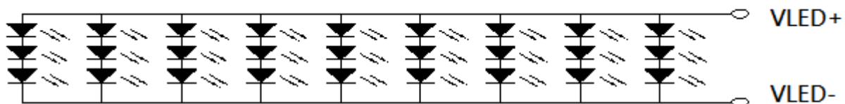
Backlight LED Circuit
