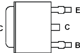
Pin Out Configuration Top View
