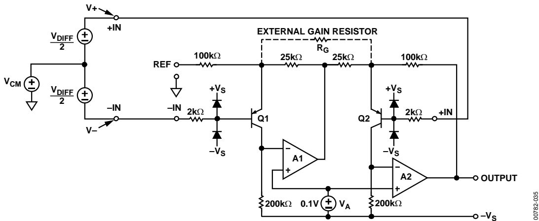
Figure 37. Amplifying Differential Signals with a Common-Mode Component
