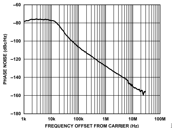
Figure 14. Closed-Loop Phase Noise, RF_{OUTB} = 10 GHz, 2x VCO, VCO = 5.0 GHz, f_{PPD} = 61.44 MHz, Loop Bandwidth = 10 kHz
