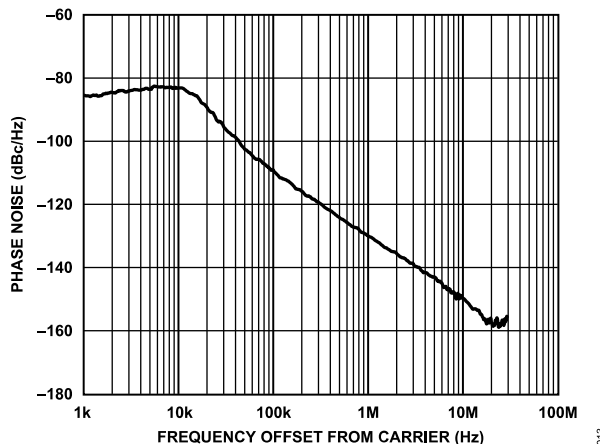
Figure 13. Closed-Loop Phase Noise, RF_{OUTB} = 6.8 GHz, 2x VCO, VCO = 3.4 GHz, f_{PPD} = 61.44 MHz, Loop Bandwidth = 10 kHz
