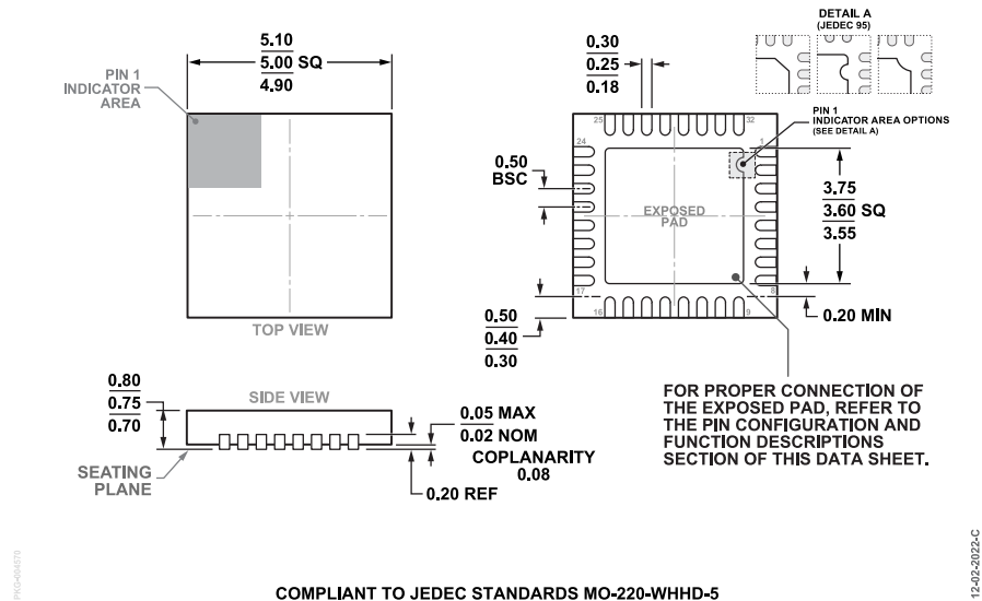
Figure 55. 32-Lead Lead Frame Chip Scale Package [LFCSP] 5 mm x 5 mm Body and 0.75 mm Package Height (CP-32-12) Dimensions shown in millimeters
