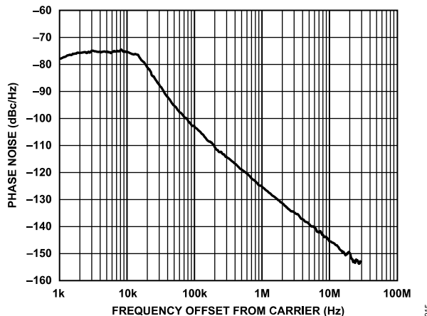
Figure 15. Closed-Loop Phase Noise, RF_{OUTB} = 13.6 GHz, 2x VCO, VCO = 6.8 GHz, f_{PPD} = 61.44 MHz, Loop Bandwidth = 10 kHz
