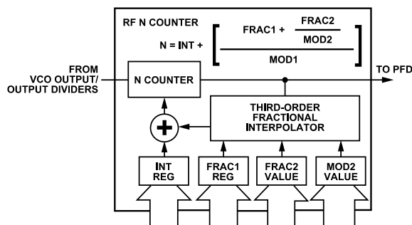
Figure 30. RF N Divider
