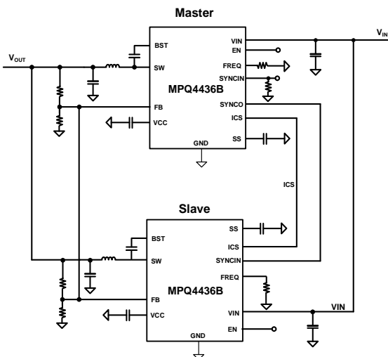
Figure 6: Dual-Phase Configuration
