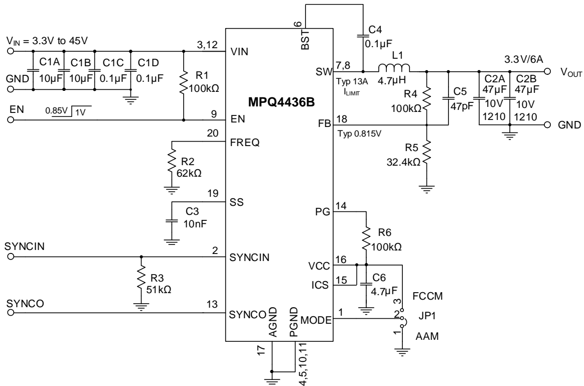
Figure 13: Typical Single-Phase Application Circuit ( V_{OUT} = 3.3V , f_{SW} = 470kHz )
