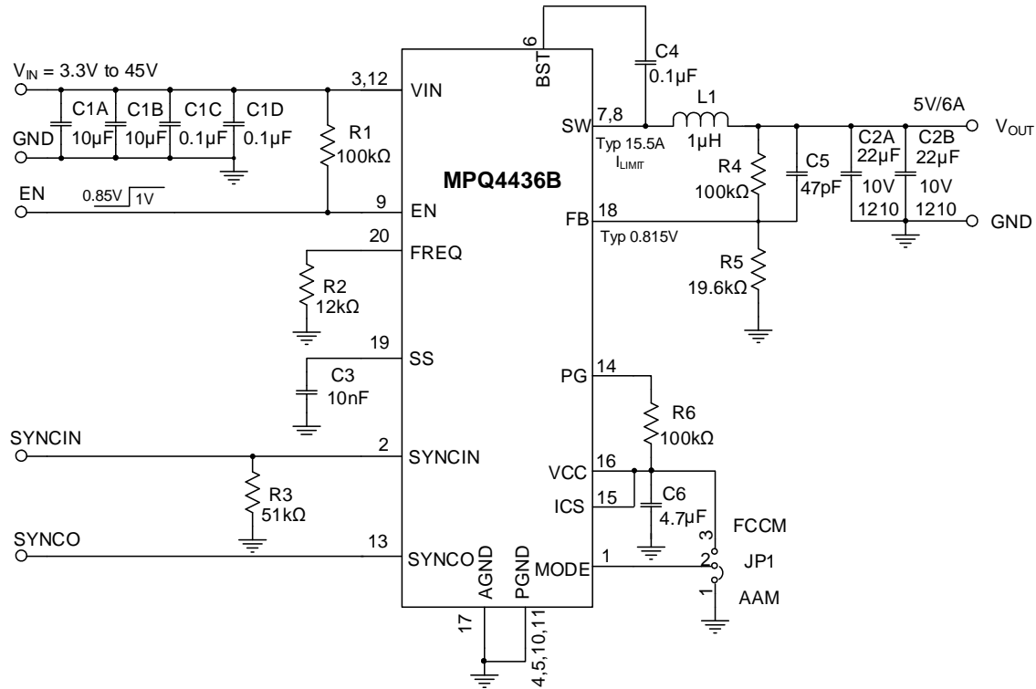
Figure 12: Typical Single-Phase Application Circuit ( V_{OUT} = 5V , f_{SW} = 2.2MHz )
