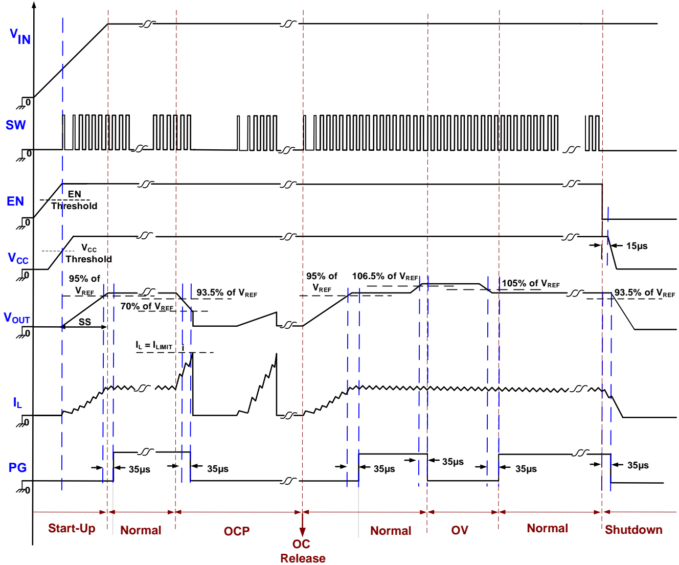
Figure 2: Timing Sequence
