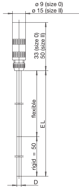
Type 902240/20
