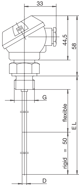
Type 902230/40
