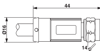
Dimensioned drawing
