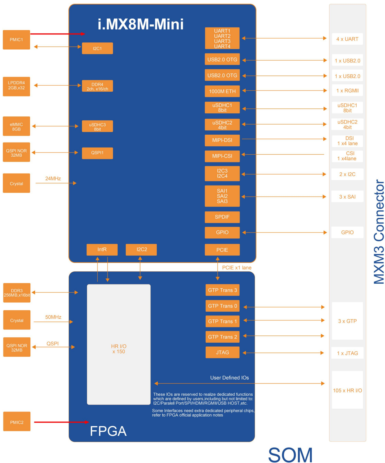
Figure 1-8 MYC-JX8MMA7 CPU Module Function Block Diagram
