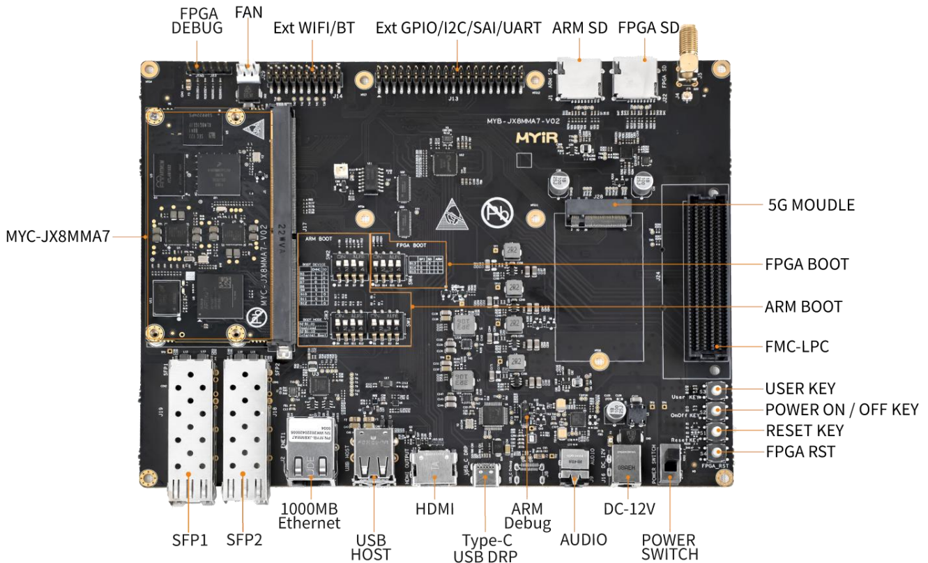
Figure 1-2 MYD-JX8MMA7 Development Board Top-view
