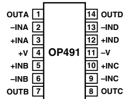
14-Lead SO
