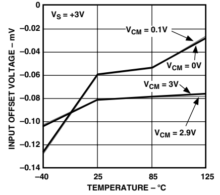
TPC 3. Input Offset Voltage vs. Temperature, V_S = +3V
