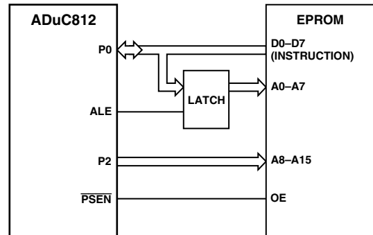
Figure 37. External Program Memory Interface
