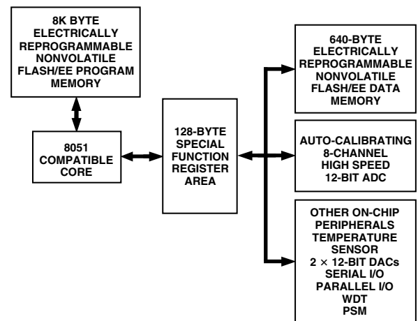
Figure 3. Programming Model
