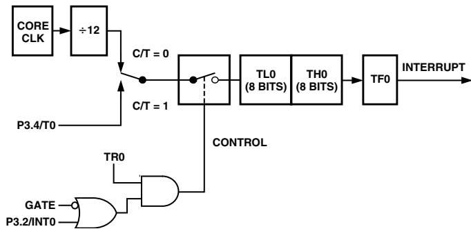
Figure 27. Timer/Counter 0, Mode 1
