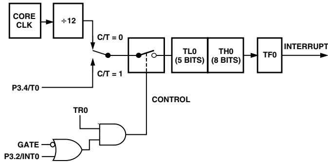
Figure 26. Timer/Counter 0, Mode 0
