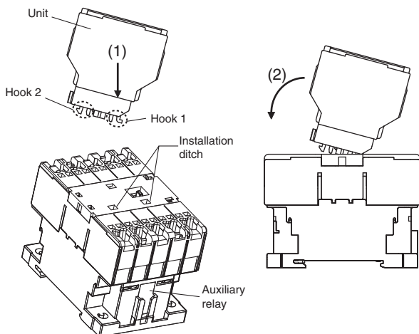
Diagram 1. Mounting method
