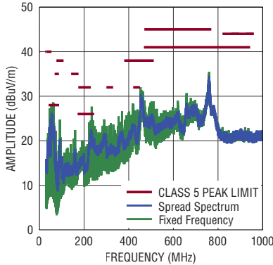
CISPR25 Radiated Emission with Class 5 Peak Limit DC2820A Demo Board V_{IN} = 14V , V_{OUT} = 5V , f_{SW} = 1.2\text{MHz} All Channels Paralleled, I_{OUT} = 12A
