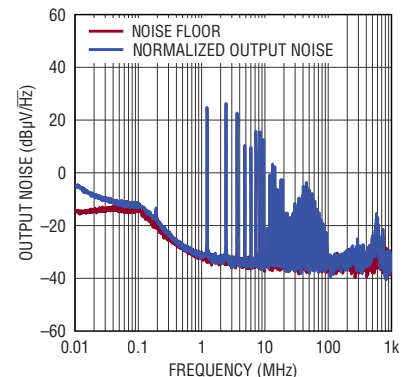
Output Noise Spectrum DC2820A Demo Board V_{IN} = 24V , V_{OUT} = 5V I_{OUT} = 3A , f_{SW} = 1.2\text{MHz}
