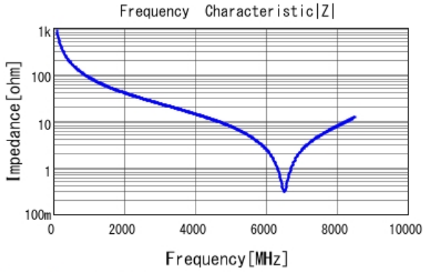
GJM1555C1H1R8BB01 |Z| DCOV, 25degC
