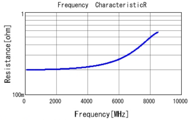
GJM1555C1H1R8BB01 R DCOV, 25degC
