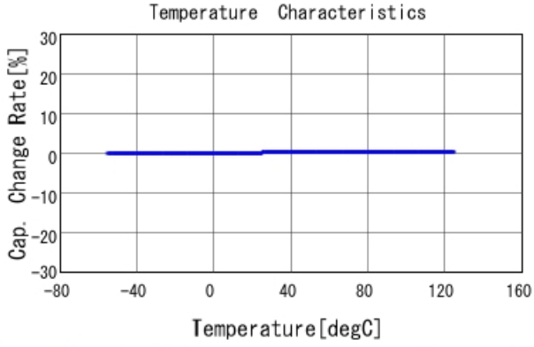
GJM1555C1H1R8BB01 C-Temp. capchange, DCOV, AC1Vrms
