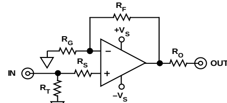
Noninverting Configuration
