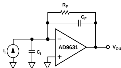
Figure 59. Transimpedance Configuration
