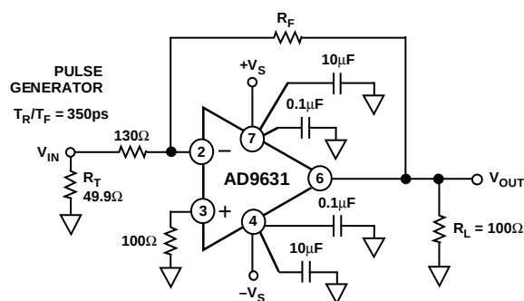
Figure 6. Inverting Configuration, G = -1
