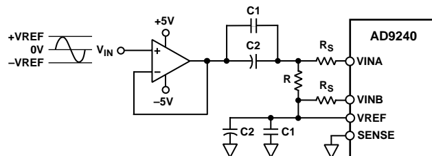
Figure 37. AC-Coupled Input
