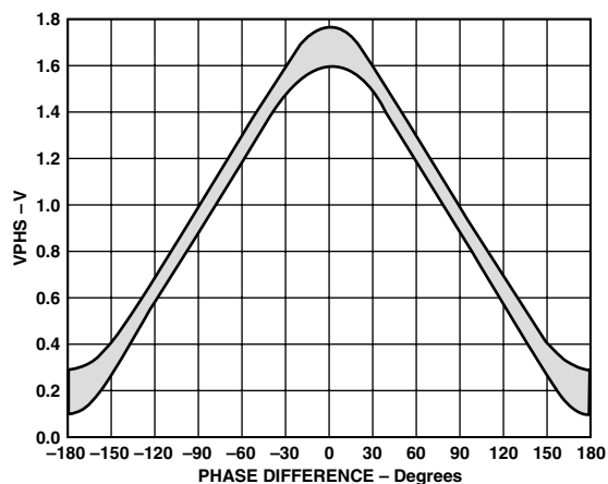
TPC 33. Distribution of VPHS vs. Input Phase Difference, Three Sigma to Either Side of Mean, Frequency 900 MHz, Temperature between -40°C and +85°C, Input Levels -30 dBm
