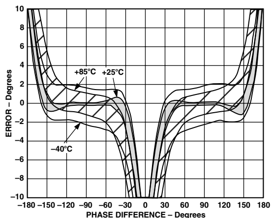
TPC 32. Distribution of VPHS Error vs. Input Phase Difference, Three Sigma to Either Side of Mean, Frequency 2200 MHz, -40°C, +25°C, and +85°C, Input Levels -30 dBm
