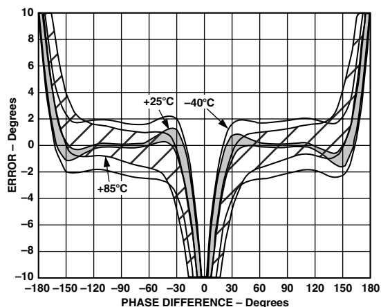
TPC 31. Distribution of VPHS Error vs. Input Phase Difference, Three Sigma to Either Side of Mean, Frequency 1900 MHz, -40°C, +25°C, and +85°C, Supply 5 V, Input Levels P_{INPA} = P_{INPB} = -30 dBm
