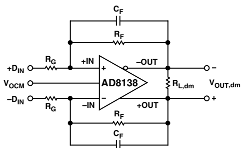
Figure 2. Circuit Definitions
