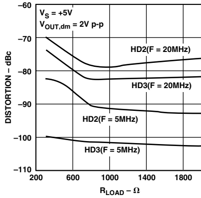
TPC 13. Harmonic Distortion vs. R_{LOAD}
