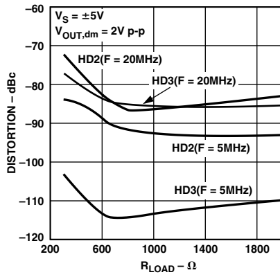
TPC 14. Harmonic Distortion vs. R_{LOAD}
