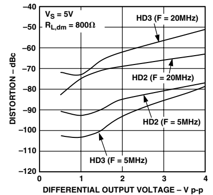
TPC 31. Harmonic Distortion vs. Differential Output Voltage, G = 2
