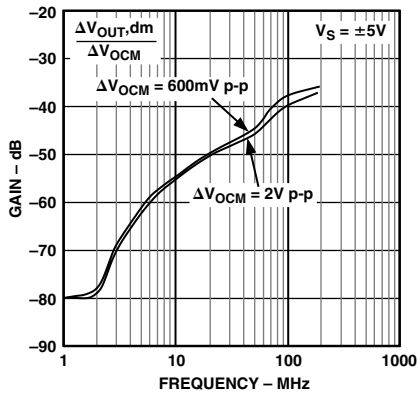
Figure 35. V_{OCM} CMRR vs. Frequency
