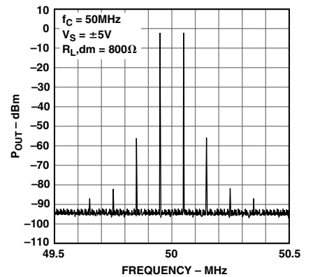
Figure 16. Intermodulation Distortion
