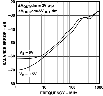
Figure 30. Output Balance Error vs. Frequency
