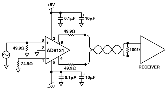
Figure 38. Single-Ended-to-Differential 100 Ω Line Driver
