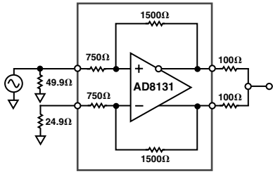
Figure 29. Output Balance Error Test Circuit
