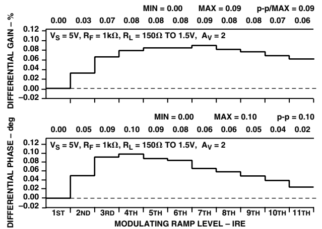
TPC 5. Differential Gain and Phase, V_S = 5V
