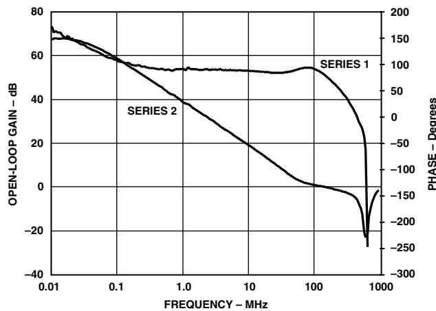
TPC 9. AD8062 Open-Loop Gain and Phase vs. Frequency, V_S = 5\text{ V} , R_L = 1\text{ k}\Omega
