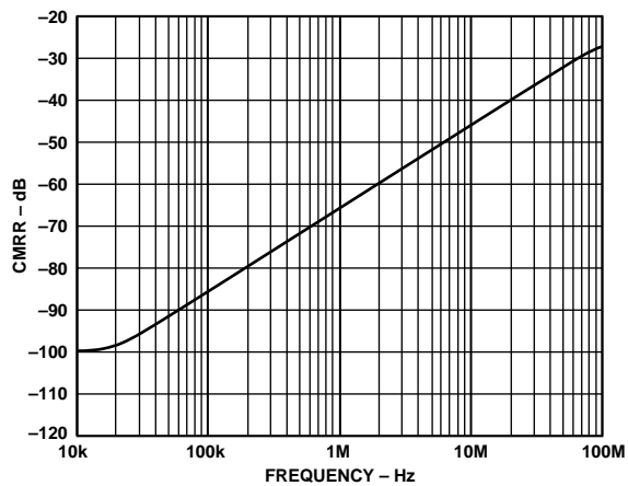
TPC 36. CMRR vs. Frequency. See Test Circuit 4.
