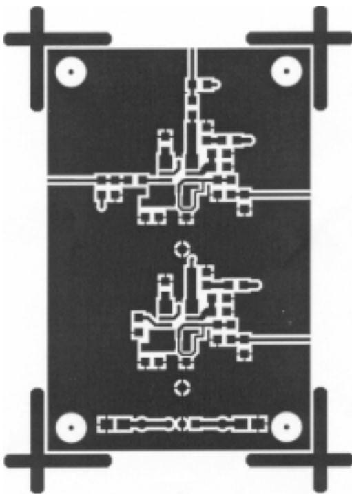
Figure 19. Evaluation Board Layout (Top)
