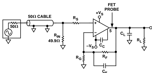
Test Circuit 2. Noninverting Gain Test Circuit with FET Probe
