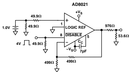
Test Circuit 6. Enable/Disable Test Circuit
