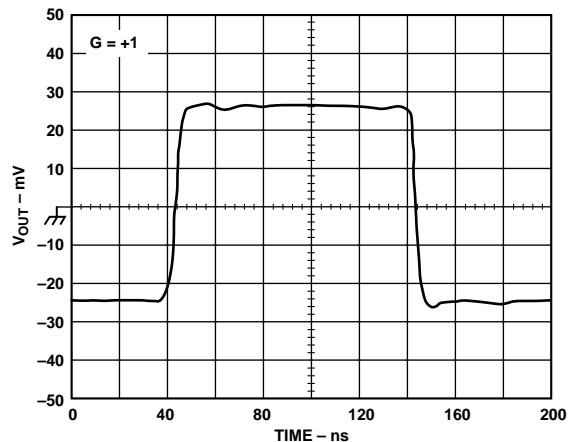
TPC 31. Small Signal Transient Response, V_O = 50\text{ mV p-p} . G = +1 . See Test Circuit 1.
