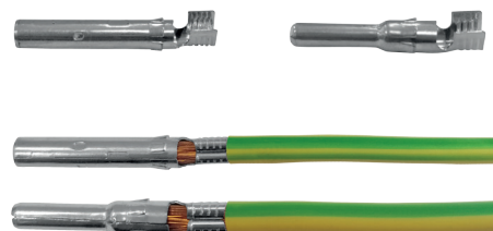
Photovoltaic connector lug pressed on a cable
