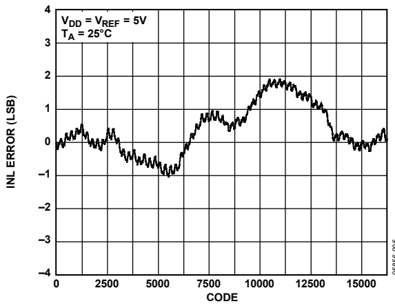
Figure 6. AD5644R INL, External Reference
