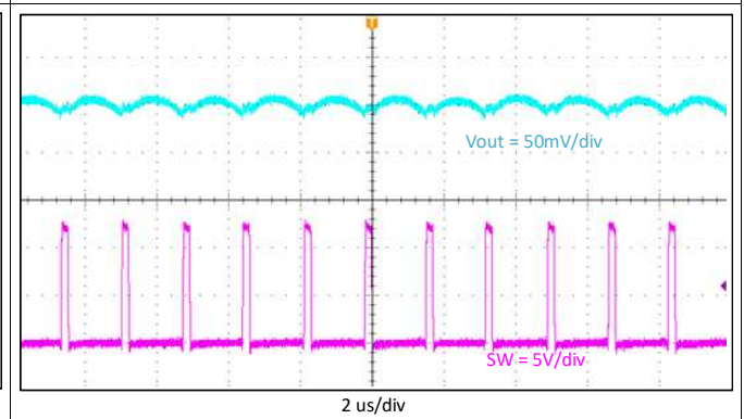
Figure 21. Output Voltage Ripple, I_{out} = 3 \text{ A}
