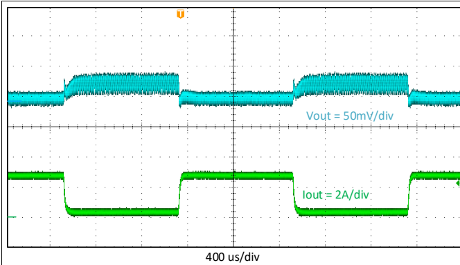
Figure 22. Transient Load Response, 0.3 to 2.7 A
