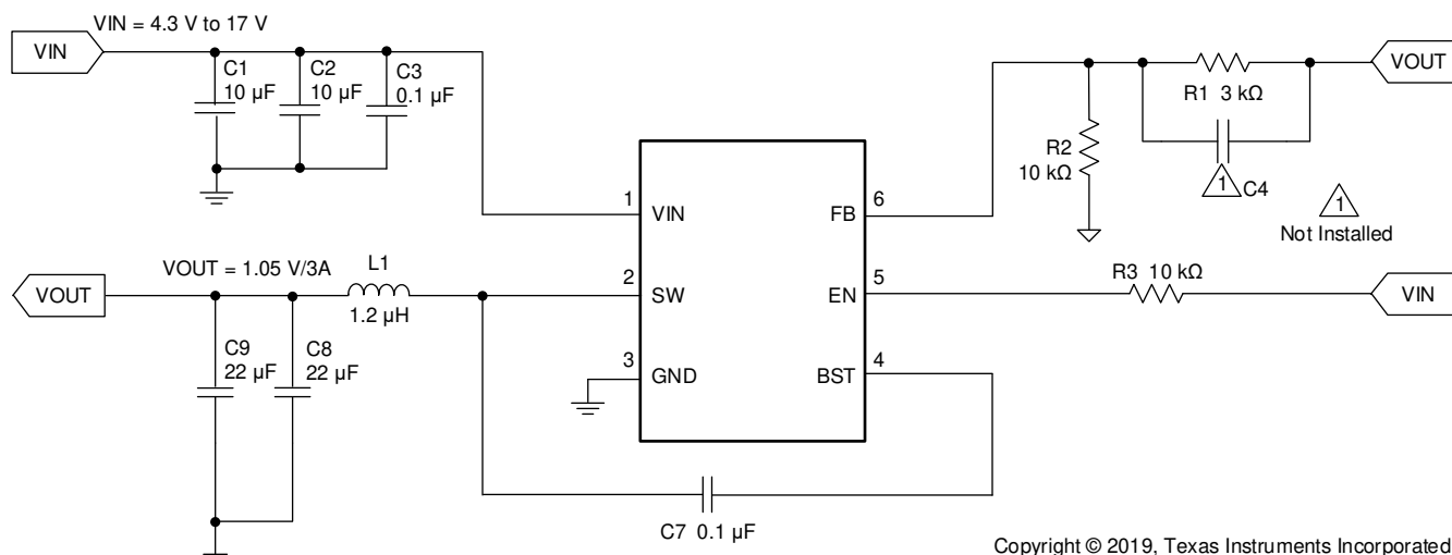
Figure 15. TPS563202 1.05-V/3-A Reference Design
