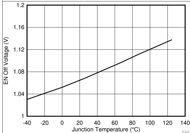
Figure 3. EN Pin EN Off Voltage vs Junction Temperature
