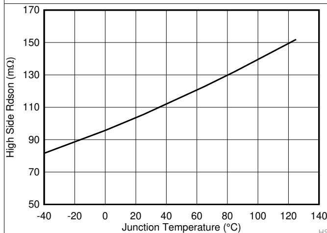
Figure 5. High-Side R_{ds-On} vs Junction Temperature
