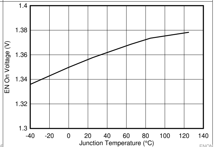
Figure 4. EN Pin EN On Voltage vs Junction Temperature
