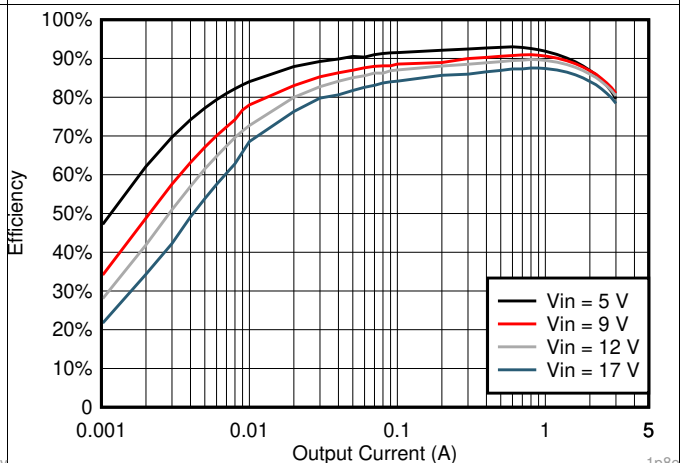
Figure 12. V_{OUT} = 1.8\text{ V} Efficiency, L = 2.2\ \mu\text{H}
