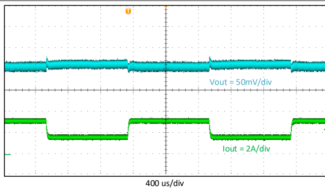
Figure 23. Transient Load Response, 1.5 to 3 A
