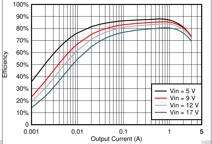
Figure 10. V_{OUT} = 1.05\text{ V} Efficiency, L = 1.2\ \mu\text{H}
