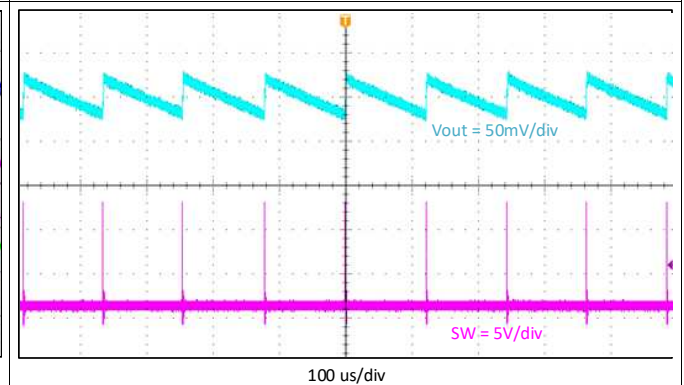
Figure 19. Output Voltage Ripple, 10 mA
