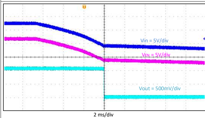
Figure 26. Shutdown Relative to V_{IN}
