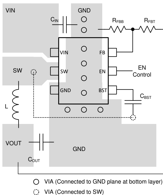
Figure 28. TPS563202 Layout
