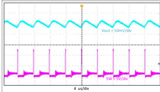
Figure 20. Output Voltage Ripple, I_{out} = 0.3 \text{ A}
