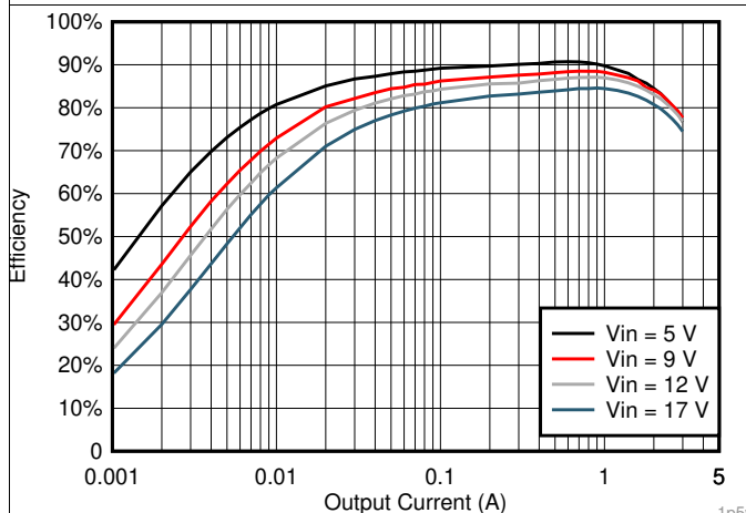
Figure 11. V_{OUT} = 1.5\text{ V} Efficiency, L = 1.5\ \mu\text{H}
