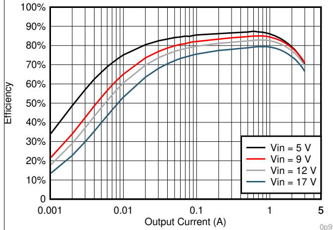
Figure 9. V_{OUT} = 0.95\text{ V} Efficiency, L = 1.2\ \mu\text{H}
