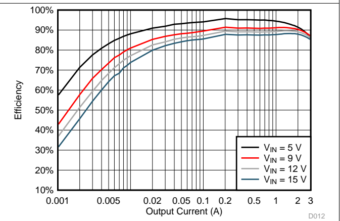
Figure 10. TPS563201 V_{OUT} = 1.5\text{ V} Efficiency, L = 2.2\ \mu\text{H}
