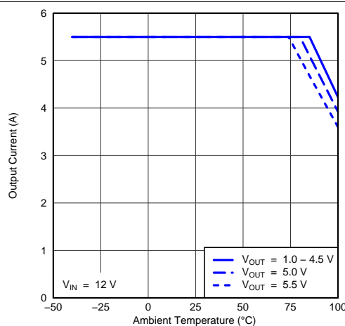
Figure 6. Output Current vs Ambient Temperature
