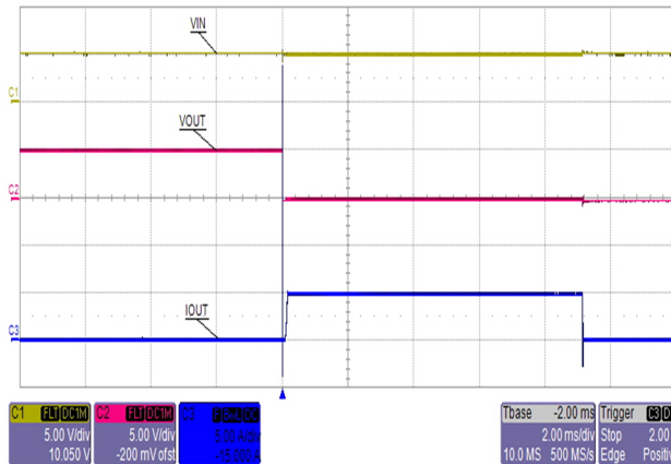
Figure 72. V_{BUS} Short-to-Ground Protection
