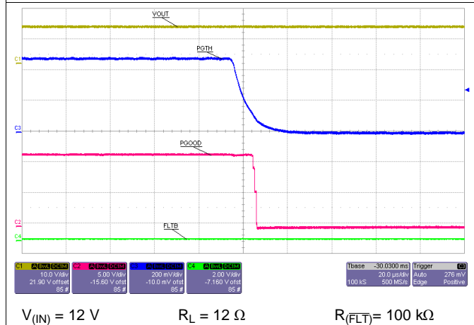
Figure 39. Power Good Delay (Falling)
