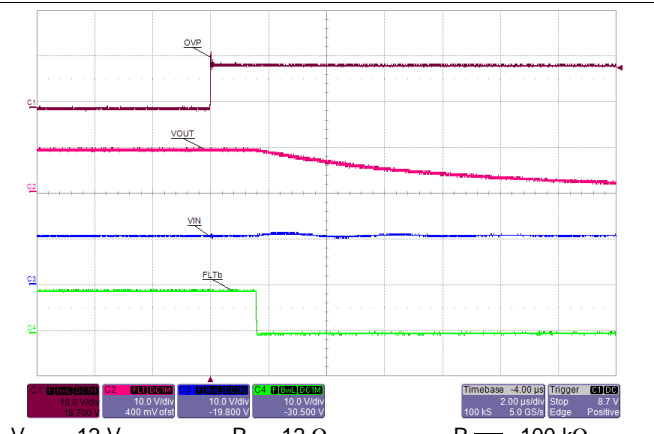
Figure 36. OVP Turn OFF Delay: OVP ↑ to Fault ↓
