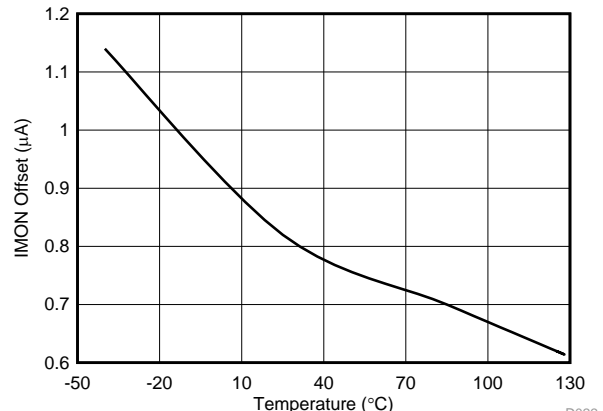
Figure 24. IMON Offset vs Temperature
