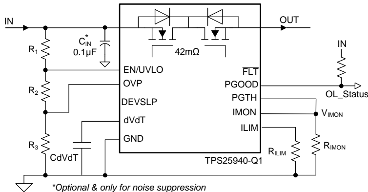
Figure 77. Circuit Configuration for Overload Detection Using TPS25940-Q1
