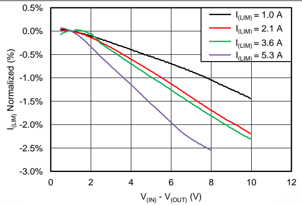
Figure 20. Current Limit Normalized (%) vs V_{(IN)} - V_{(OUT)} Thermal shutdown occurs when I_{(LIM)} = 5.3\text{ A} and [V_{(IN)} - V_{(OUT)}] > 8\text{ V}
