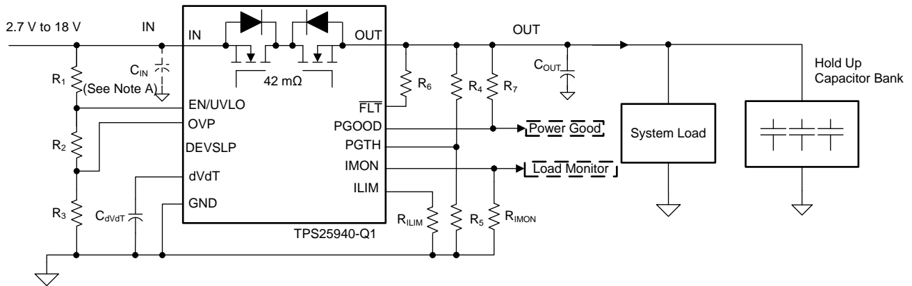
Figure 73. Holdup Capacitor Implementation Using TPS25940-Q1
