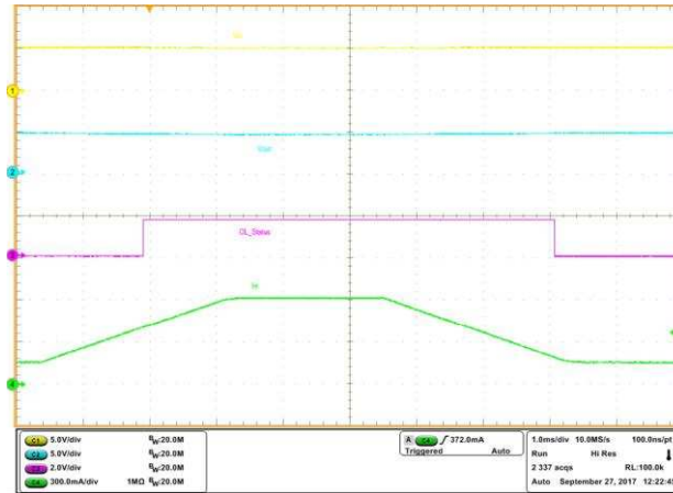
Figure 78. Overload Flag Status for Change in Load from 150 mA to 600 mA and Back
