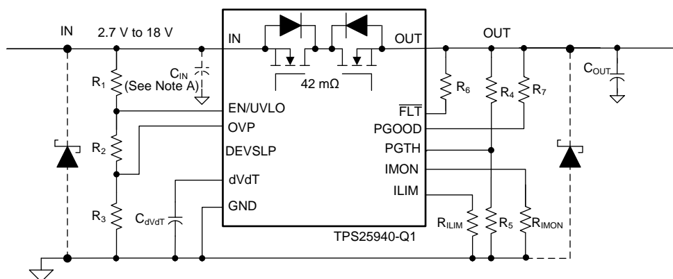
Figure 79. Circuit Implementation with Optional Protection Components
