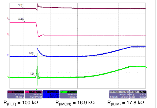
Figure 40. Hot-Short: Fast Trip Response and Current Regulation
