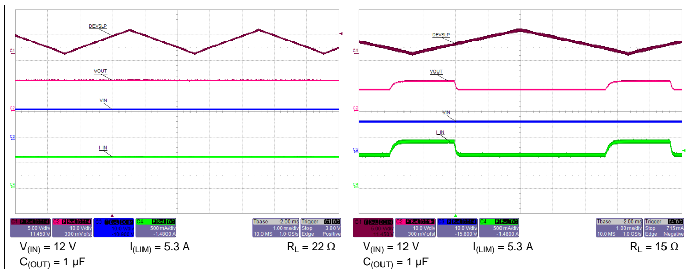
Figure 46. IN and OUT of DevSleep Mode with 550-mA Load
