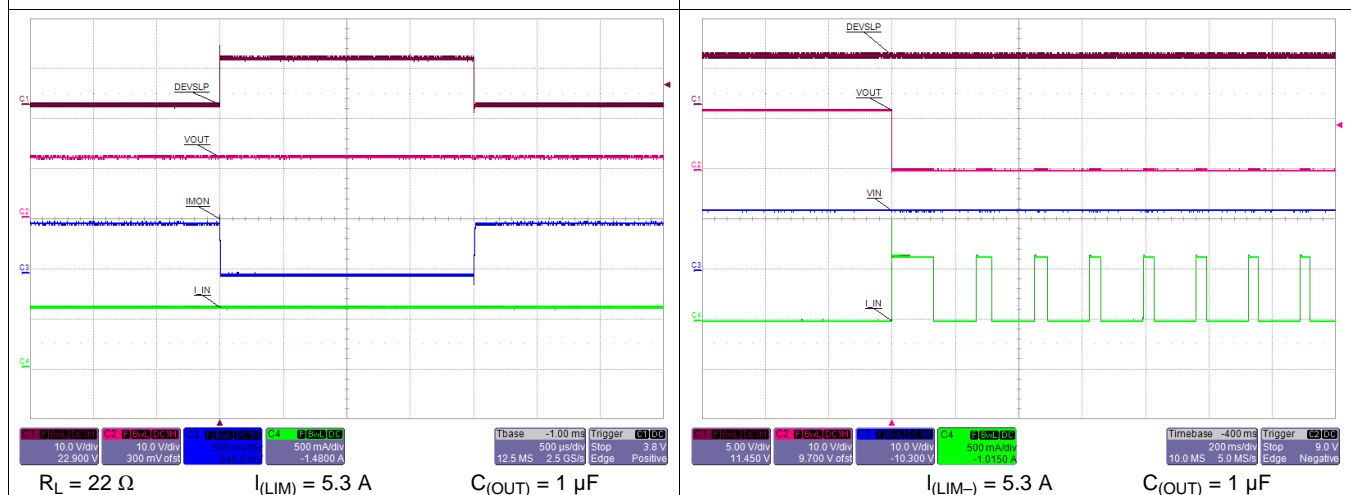
Figure 47. IN and OUT of DevSleep Mode with 800-mA Load. In DevSleep, Load Current gets Limited to I_{(DEVSLP(LIM))}
