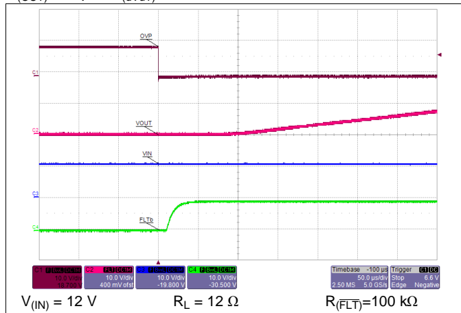
Figure 37. OVP Turn ON Delay: OVP ↓ to Output Ramp ↑
