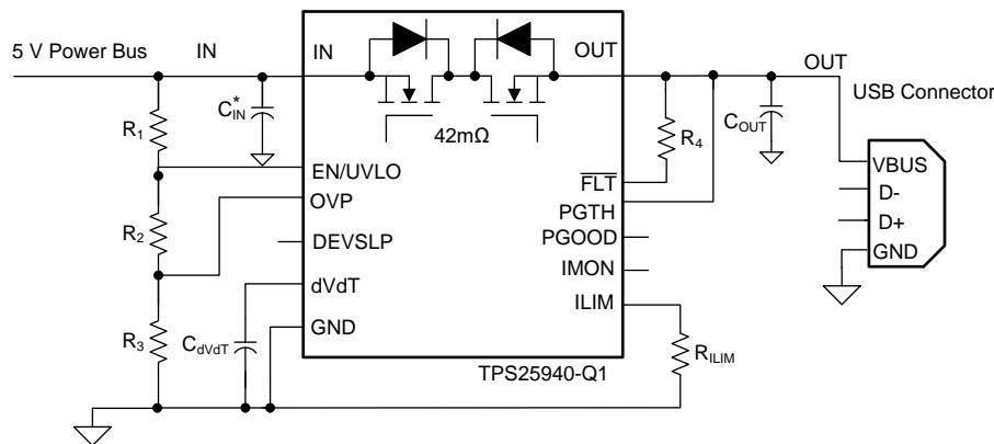
Figure 70. Automotive USB Hub-Port – V_{BUS} Short to Battery, V_{BUS} Short to GND Protection
