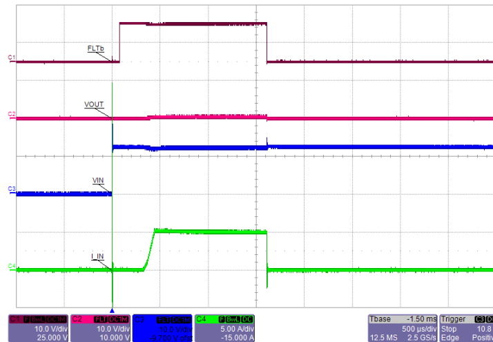
Figure 69. Hot Plug-in with Short on Output: Latched - TPS25940L-Q1
