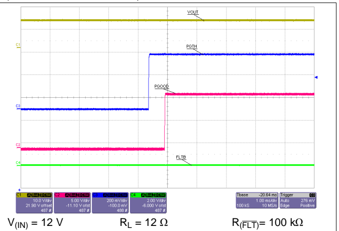
Figure 38. Power Good Delay (Rising)
