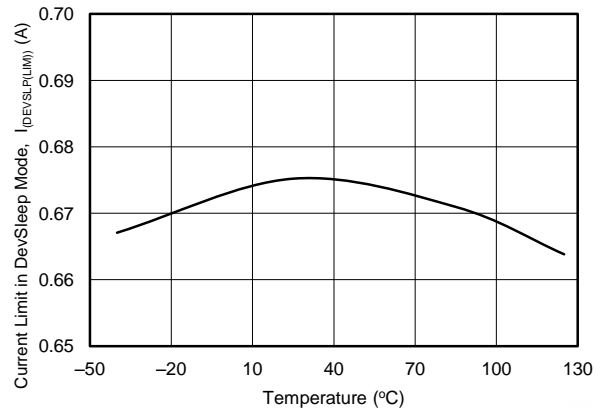
Figure 22. Current Limit in DevSleep Mode vs Temperature
