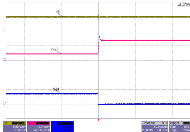
Figure 71. V_{BUS} Short-to-Battery Protection
