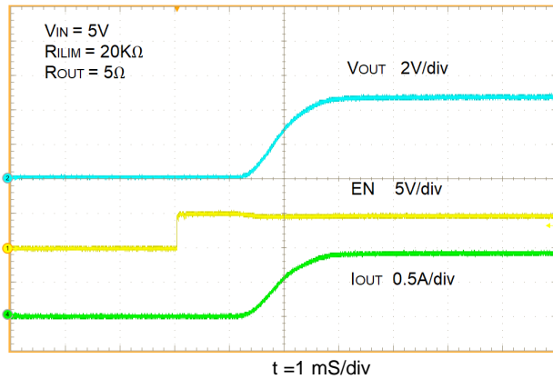
Figure 1. Turnon Delay and Rise Time
