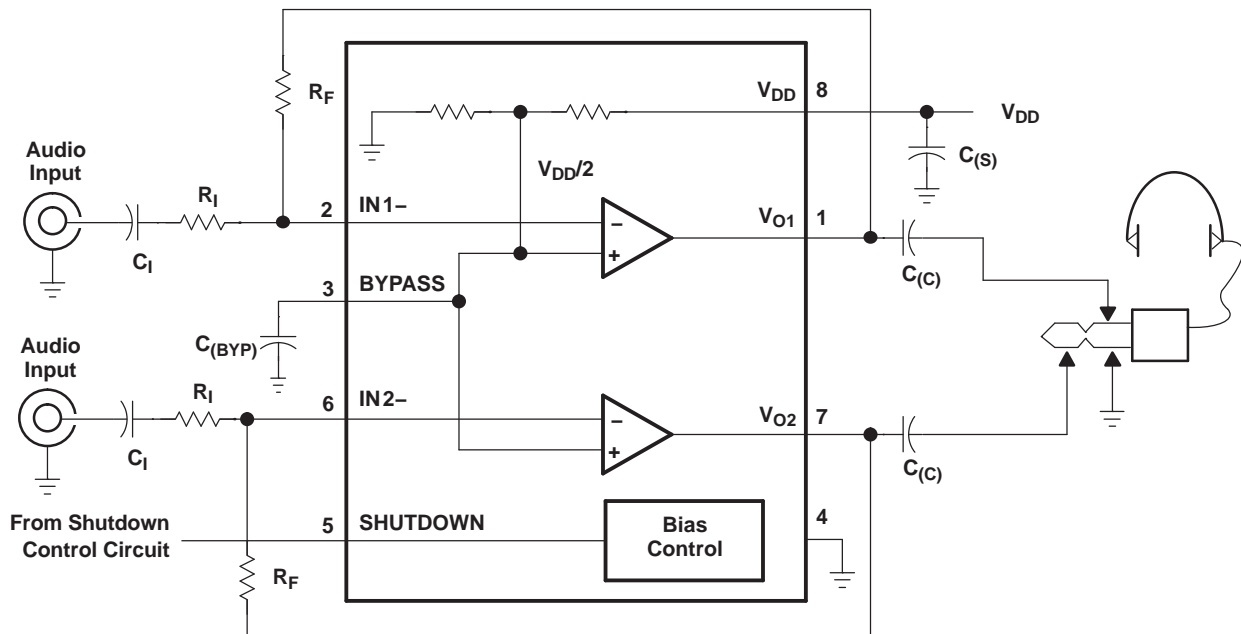
Figure 35. Typical Application
