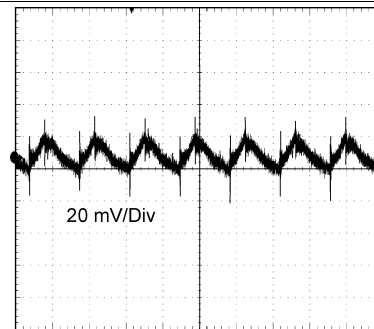
Figure 34. Output Ripple
