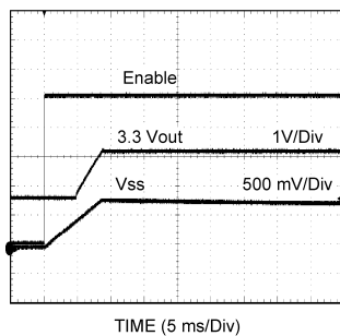
Figure 48. Prebiased Start-Up
