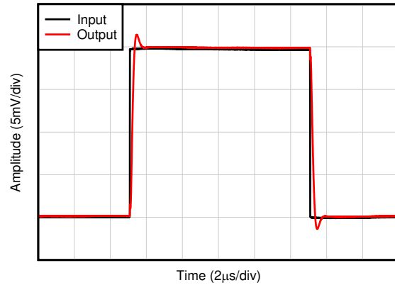
Time (2µs/div) C_L = 20\text{ pF} , G = 1 , 20-mV step response
