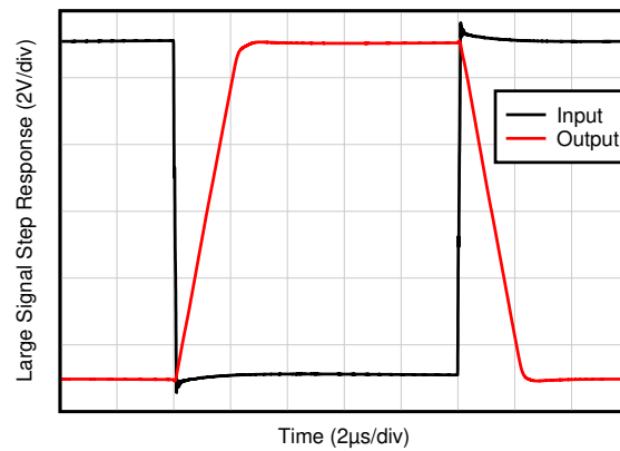
Time (2µs/div) C_L = 10\text{ pF} , G = -1
