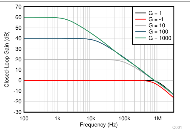
Figure 6-8. Closed-Loop Gain and Phase vs Frequency
