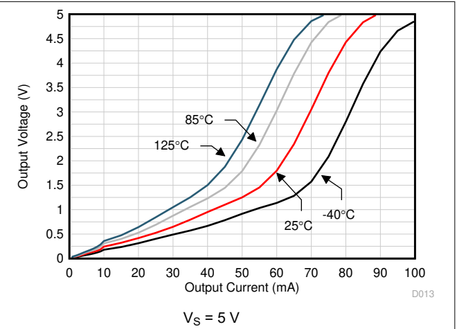
Figure 6-14. Output Voltage Swing vs Output Current (Sinking)
