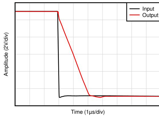
Time (1µs/div) C_L = 20\text{ pF} , G = 1
