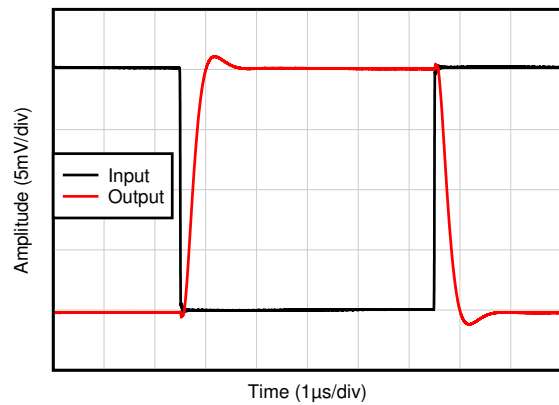
Time (1µs/div) R_L = 1\text{ k}\Omega , C_L = 20\text{ pF} , G = -1 , 10-mV step response
