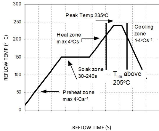
Figure 15: Reflow Profile for Tin/Lead (Sn/Pb) process.
