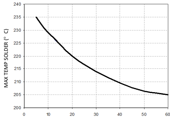
Figure 16: Time Limit Curve Above 205°C Reflow for Tin Lead (Sn/Pb) process.
