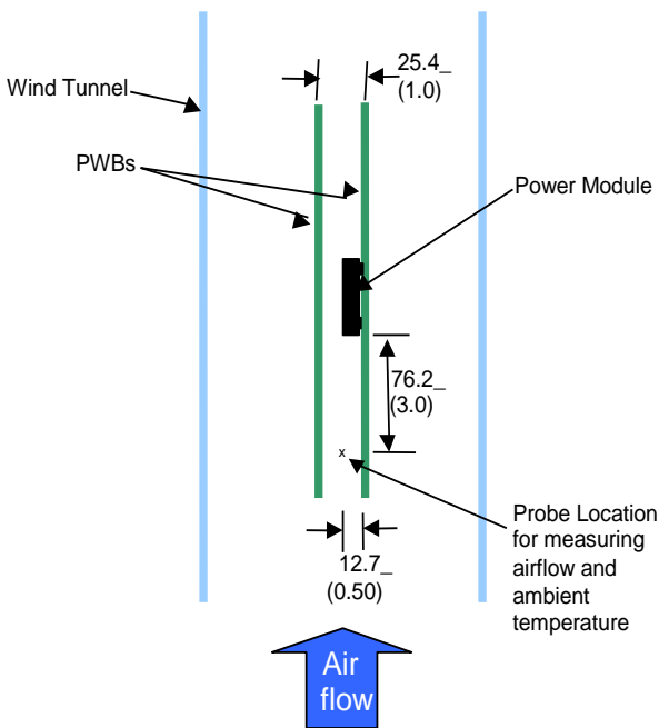
Figure 12. Thermal Test Set-up.
