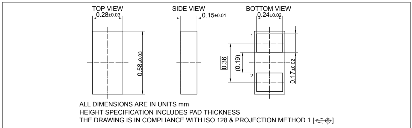
Figure 10 WLL-2-3 package
