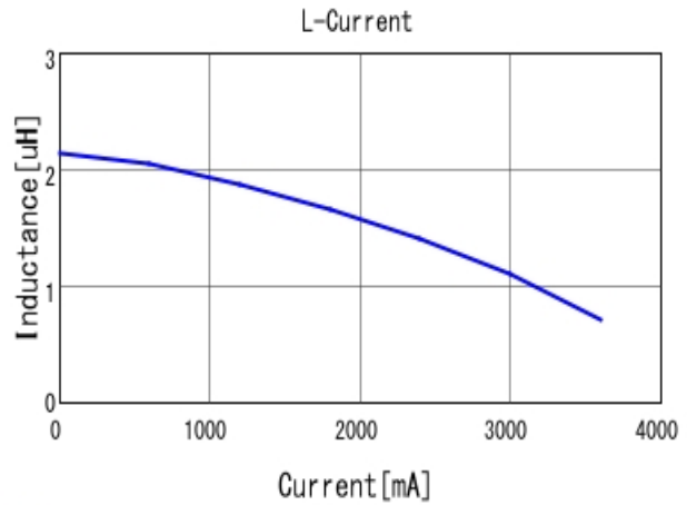
■ DFE201610P-2R2M L-Current 20degC
