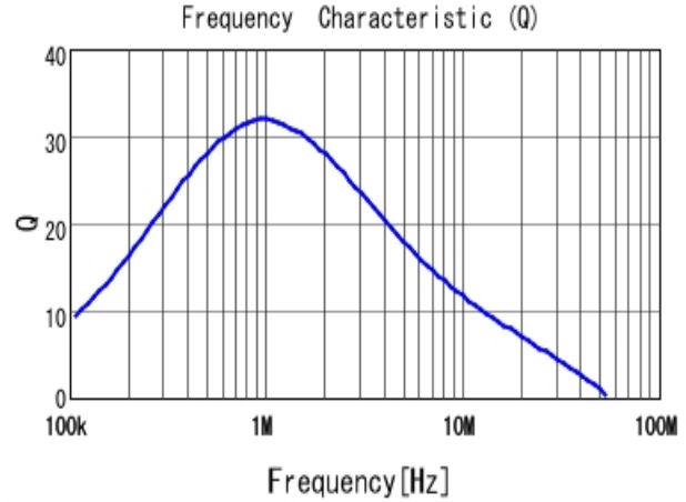
■ DFE201610P-2R2M Q
