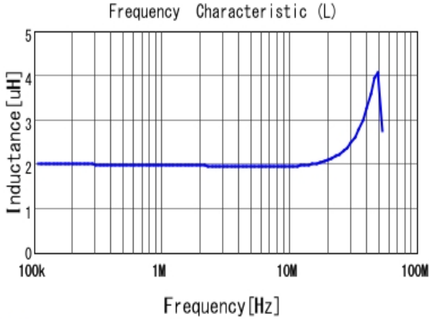
■ DFE201610P-2R2M L
