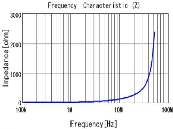
■ DFE201610P-2R2M |Z|
