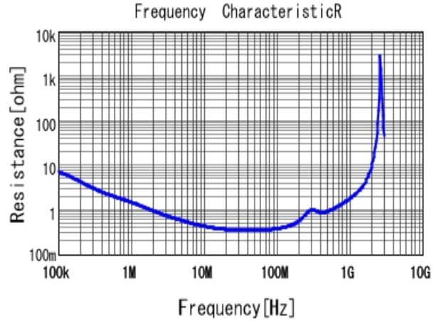
■ DE2E3KY472MN3AM02F R DCOV, 20degC
