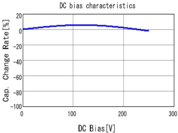
■ DE2E3KY222MA2BM01F C-DC bias capchange, 20.0degC, AC1
