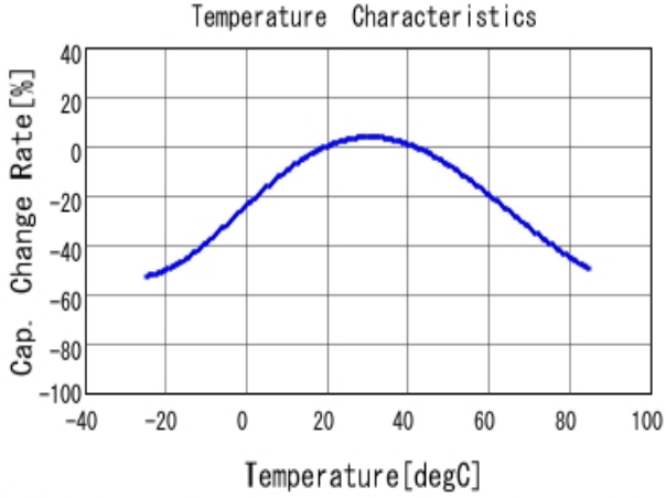
■ DE2E3KY222MA2BM01F C-Temp. capchange, DCOV, AC1Vrms
