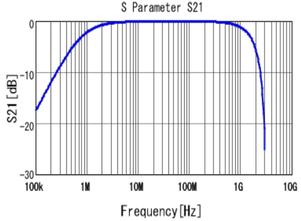
■ DE2E3KY222MA2BM01F S21 DCOV, 20degC
