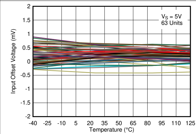
Figure 6-19. Input Offset Voltage vs. Temperature at 5V
