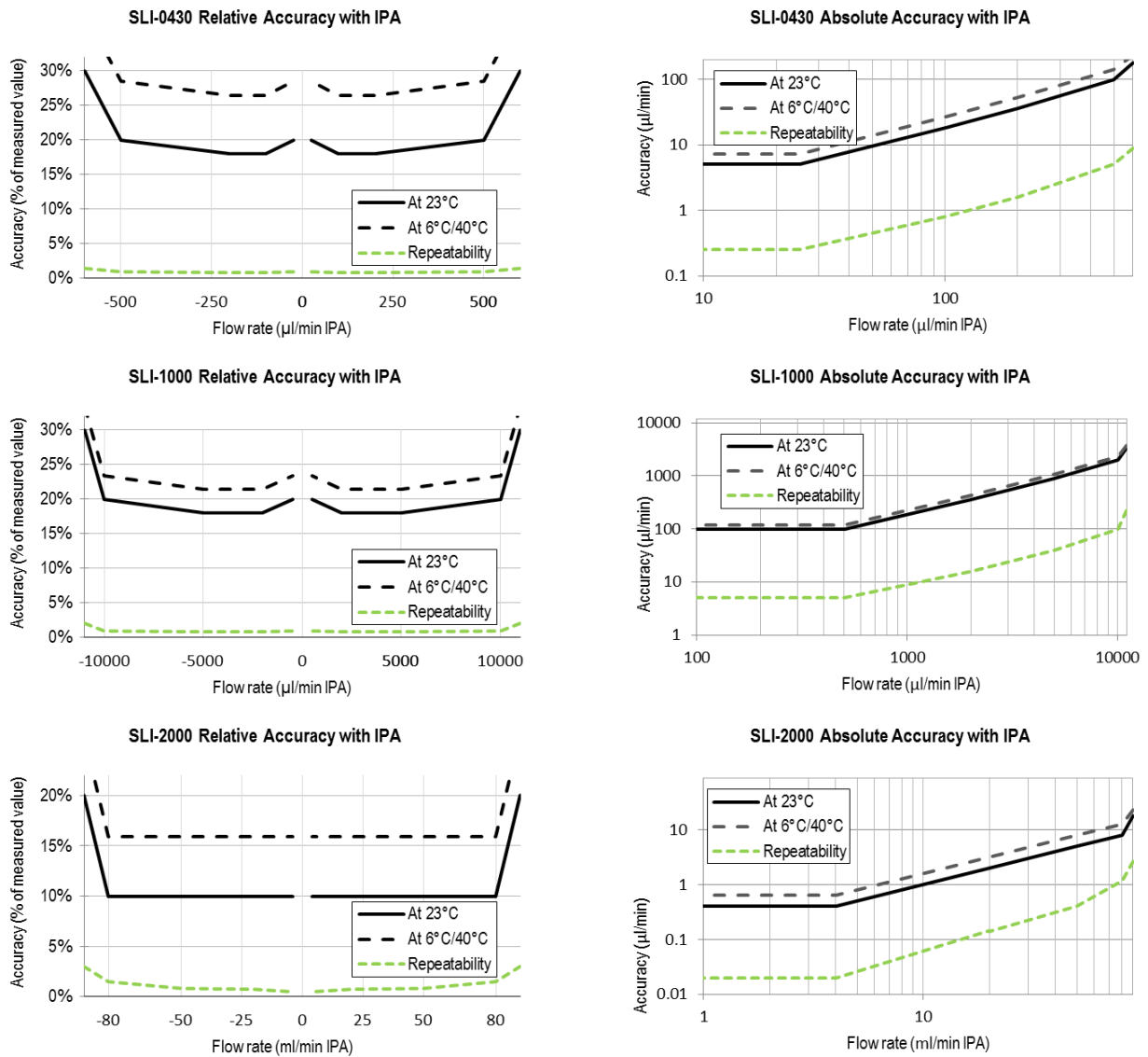
Figure 2: Flow meter accuracy and repeatability across the flow range. Relative error in % of measured value (left column) and absolute error in µl/min or ml/min in case of the SLI-2000 (right column) for IPA
