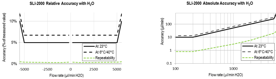
Figure 1 (cont.): Flow meter accuracy and repeatability across the flow range. Relative error in % of measured value (left column) and absolute error in µl/min (right column) for H 2 O
