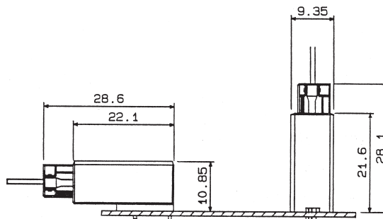
Horizontal/Vertical Type
