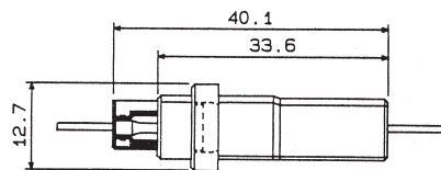
Panel/Free-Hanging Type
