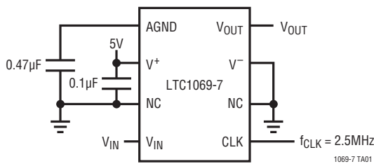
Single 5V Supply, Linear Phase 100kHz Lowpass Filter
