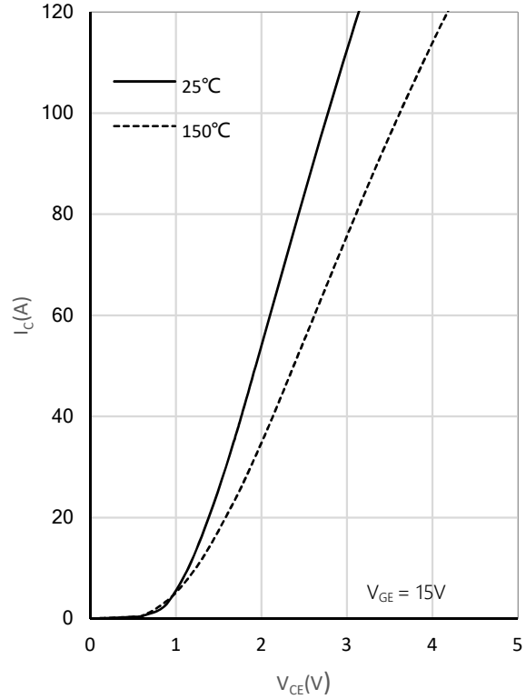
Fig. 2 Saturation voltage characteristics
