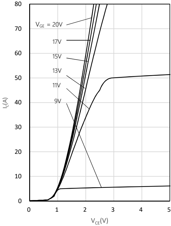
Fig. 1 Output characteristics
