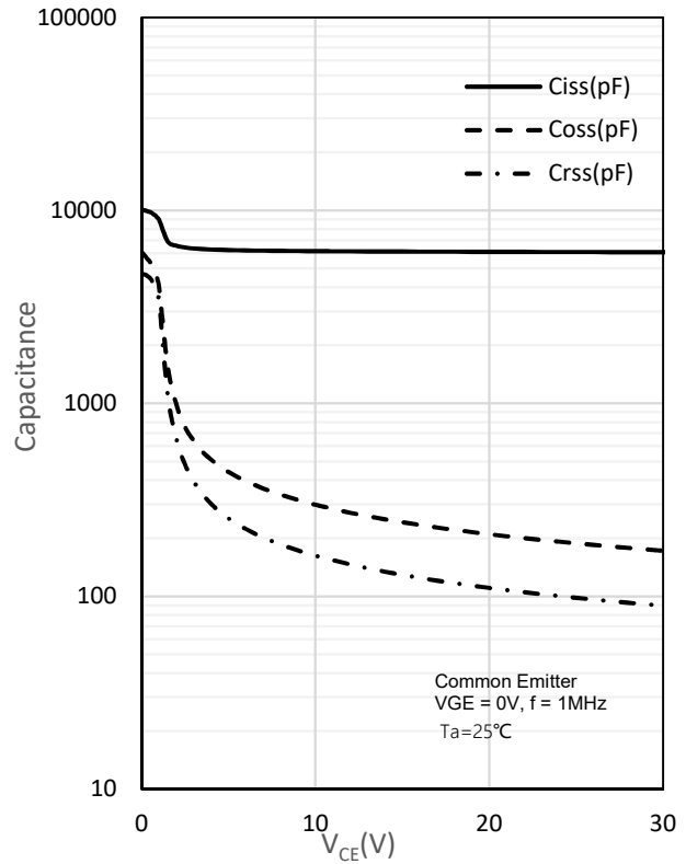
Fig. 8 Capacitance characteristics
