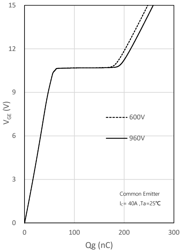
Fig. 7 Gate charge characteristics
