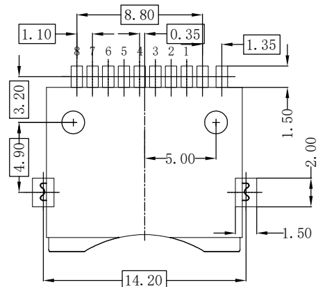
RECOMMENDED P. C. B LAYOUT (TOP VIEW) GENERAL TOLERANCE ±0.05
