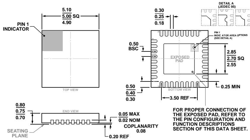
Figure 77. 32-Lead Lead Frame Chip Scale Package [LFCSP] 5 mm × 5 mm Body and 0.75 mm Package Height (CP-32-21) Dimensions shown in millimeters
